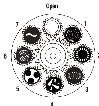
Gobo wheel with 7 rotating gobos and open
