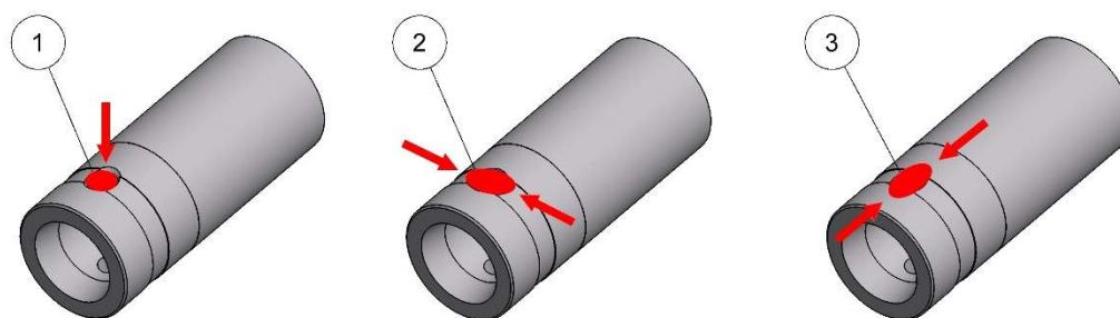
Figure 20: Conical connections.
